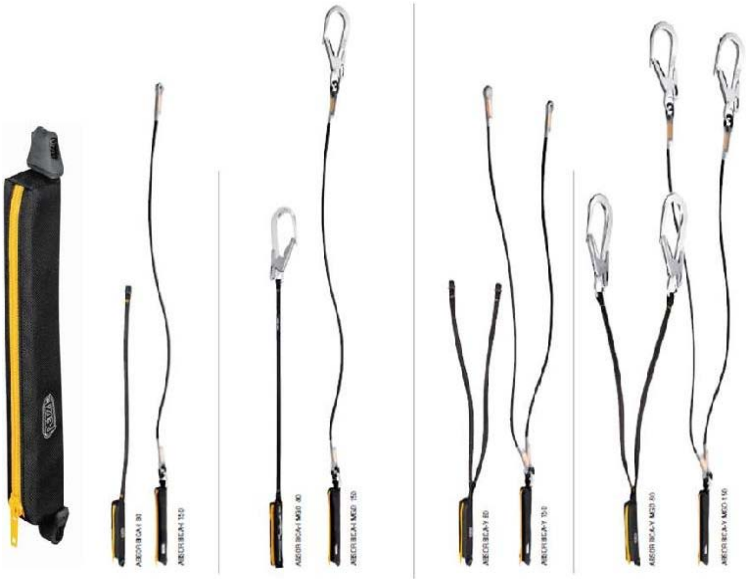
ABSORBICA L57 basic (left) and in its various configurations (right)
